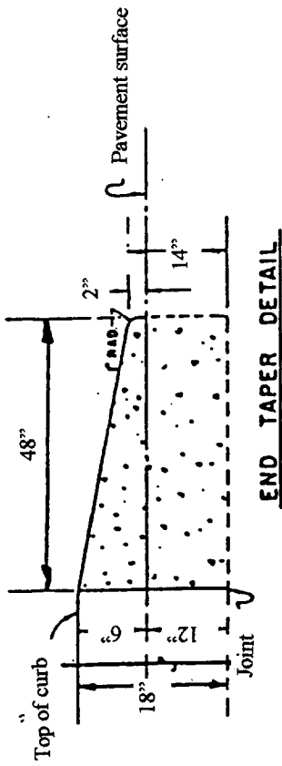
VERTICAL CURB DETAIL
