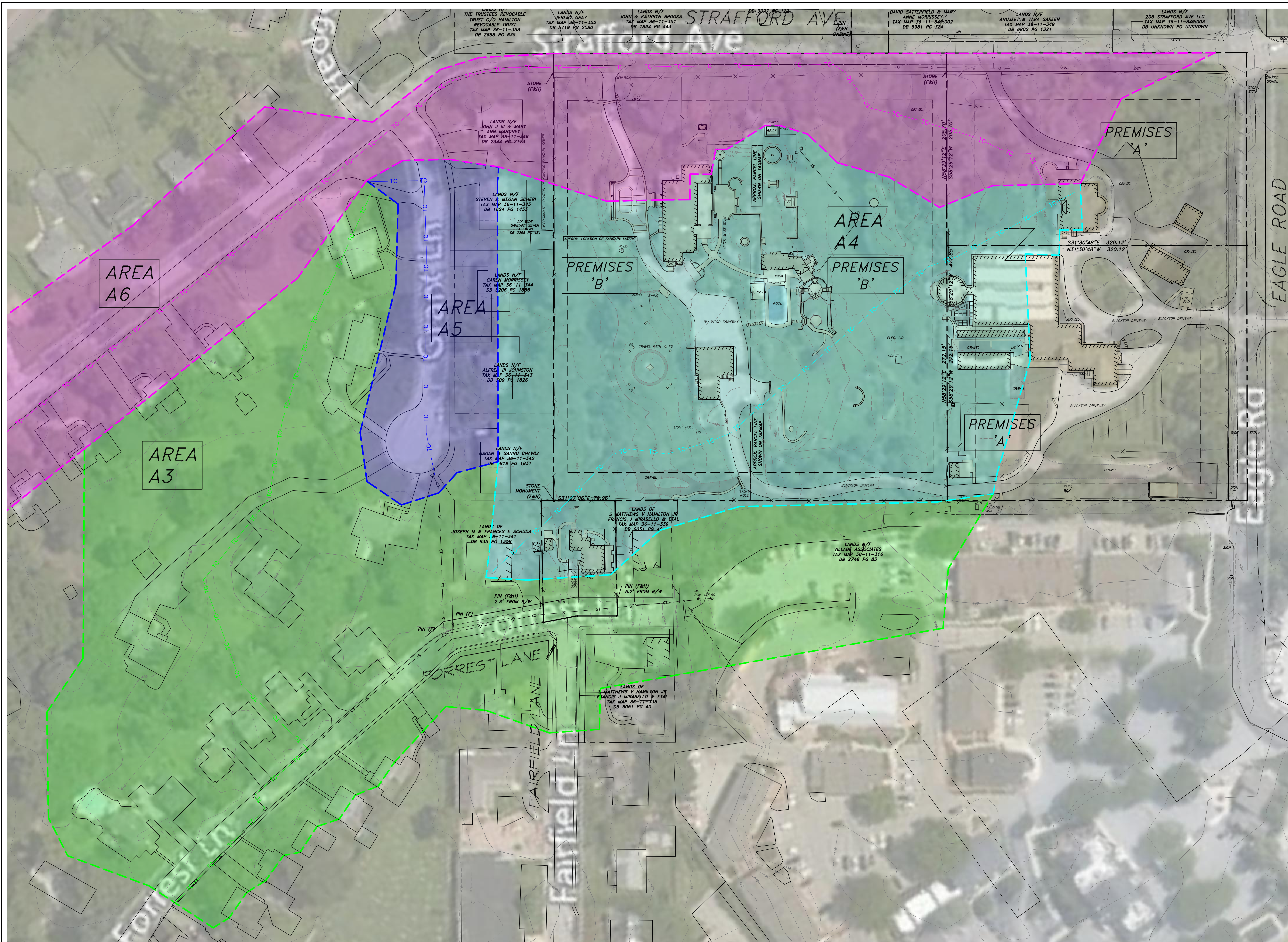
DRAINAGE AREA SUMMARY TO FORREST LN
