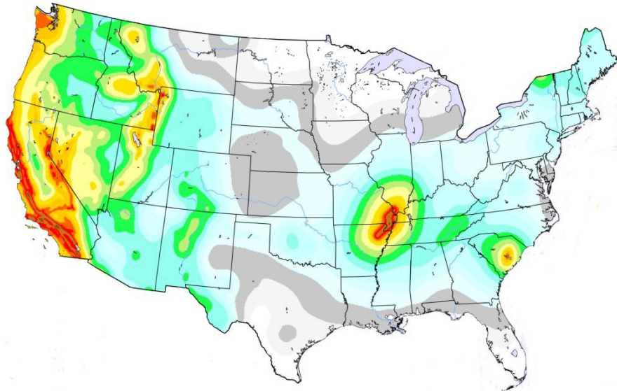
Figure 5. Seismic Risk.
